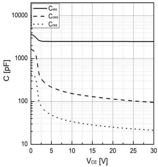
Fig 13. Typical capacitance as a function of V CE (f=1Mhz, V GE =0V)
