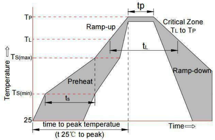
FIG.2: Reflow condition
